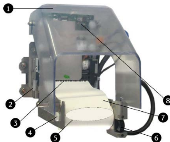
Fig. 72: Receipt printer
