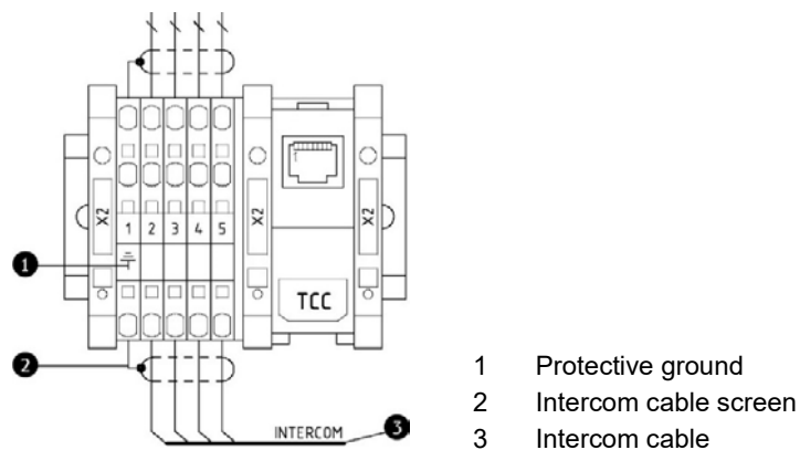
Fig. 38: Terminal block -X2, connection intercom system, with 4-wire connection
