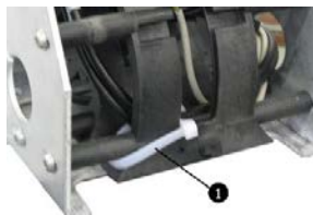
Fig. 50: Feeding channel I blocked
