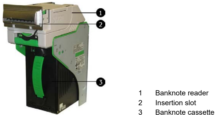
Fig. 82: Banknote processing NBA
