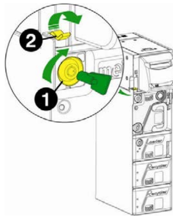
Fig. 102: Locking mechanism
