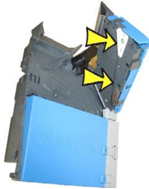
Fig. 81: Cleaning of the lower edge of the coin route
