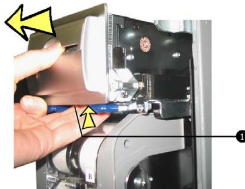
Fig. 90: Removing the banknote reader
