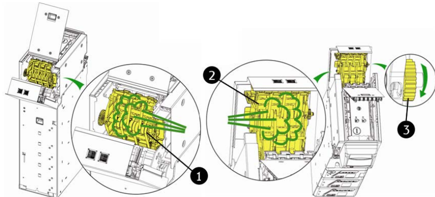
Fig. 111: Cleaning the test unit
