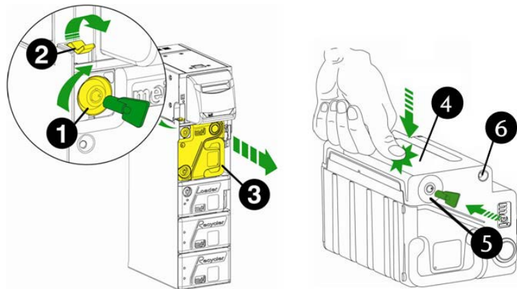
Fig. 103: Removing and opening the banknote cassette
