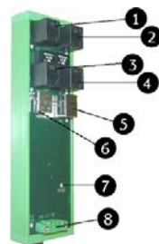
Fig. 44: Interface extension USB-4-COM
