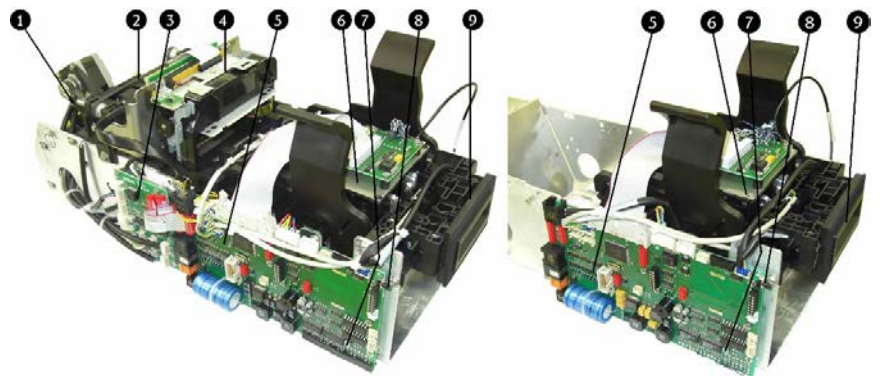
Fig. 48: Multicon with magnetic strip technology (example for equipment at ENT (left) and EXT (right))
