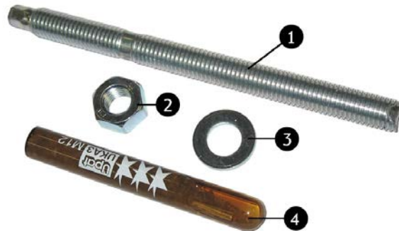
Fig. 32: DESIGNA mounting kit
