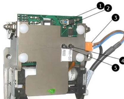
Fig. 74: PCB receipt printer
