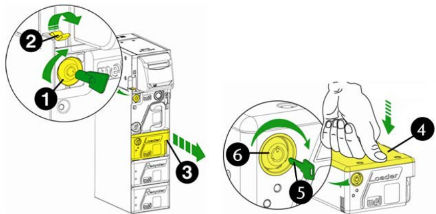
Fig. 104: Removing and opening the loader cassette
