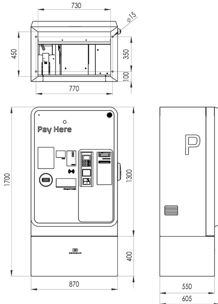
Fig. 6: Pay Cash&Card, with optional illuminated frame, dimensions in mm
