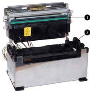
Fig. 66: Ticket printer incl. cutter
