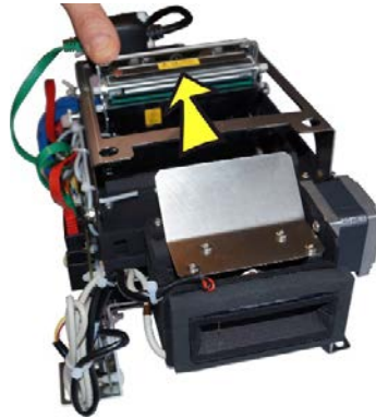
Fig. 71: Folding up the thermal line
