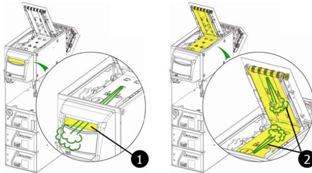
Fig. 110: Cleaning the banknote acceptor and the positioner
