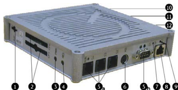
Fig. 42: TCC (Type LCC)
