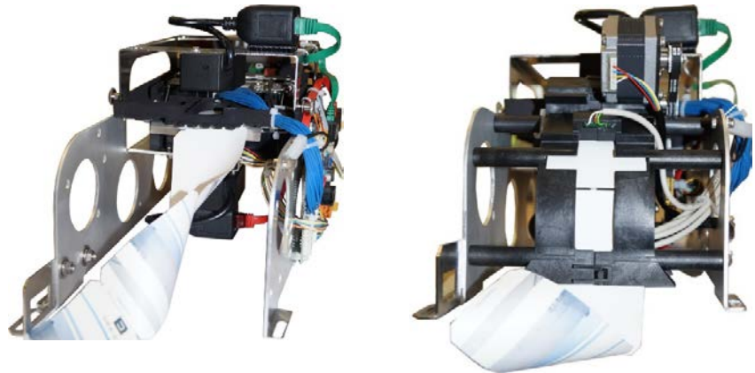
Fig. 70: Multicon MC Barcode: Without double feeding unit (left), with double feeding unit (right)
