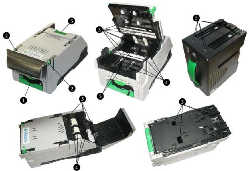
Fig. 84: Cleaning the NBA
