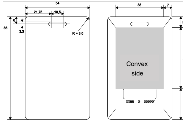
Fig. 119: EasyMove card (active): Approx. dimensions in mm
