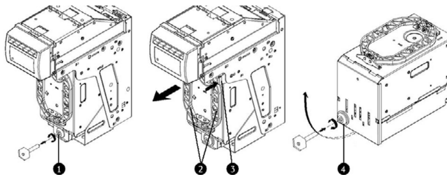
Fig. 86: Removing and opening the MFL stacker cassette (Figure with options)
