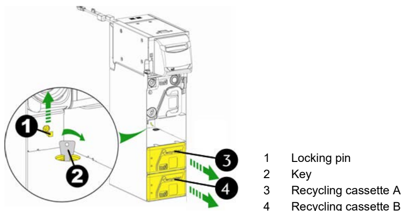
Fig. 116: Removing the recycling cassette
