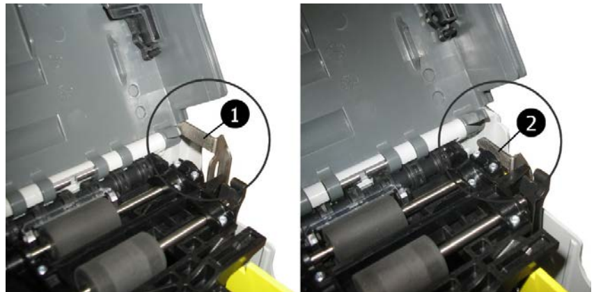
Fig. 105: Loader cassette, locking latch: correct position (left), wrong position (right)
