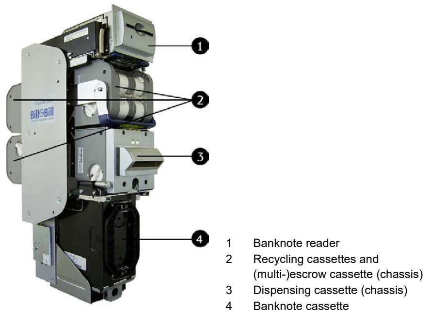
Fig. 88: Banknote recycler BNR CASHCODE
