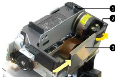
Fig. 61: Place the ribbon cartridge
