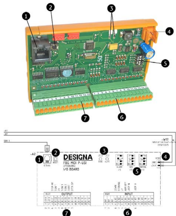
Fig. 46: I/O interface Midi-P-USI (here I/O interface assignment of an entrance control terminal)
