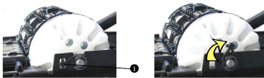
Fig. 95: Removing the path switch
