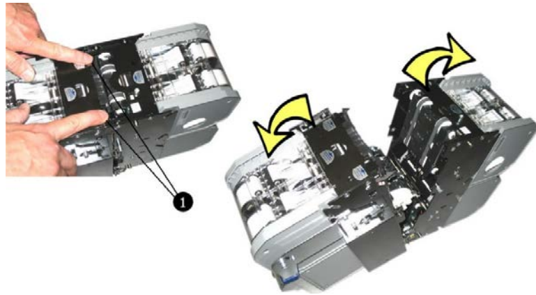
Fig. 93: Opening the chassis
