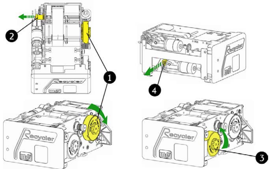
Fig. 117: Recycling cassette: Removing trapped banknotes
