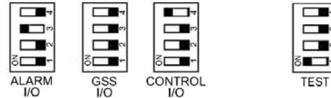
Fig. 47: DIP switch positions
