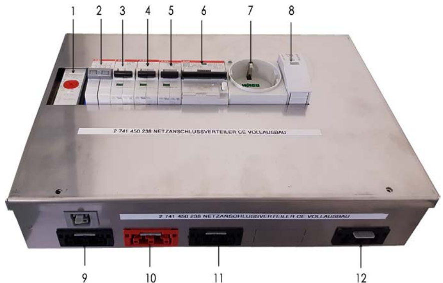
Fig. 16: Power distribution box (figure with options)
