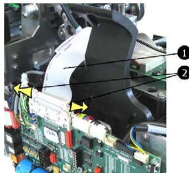
Fig. 60: Disconnecting the flat cable
