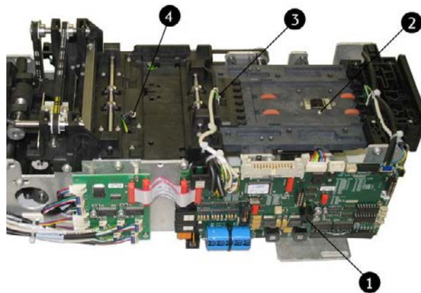
Fig. 62: Live LED and light barrier for error analysis
