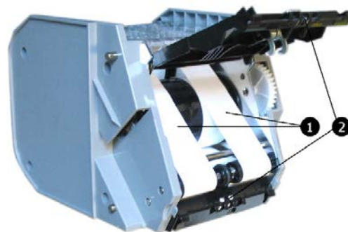
Fig. 98: Cleaning the recycling or (multi-)escrow cassettes
