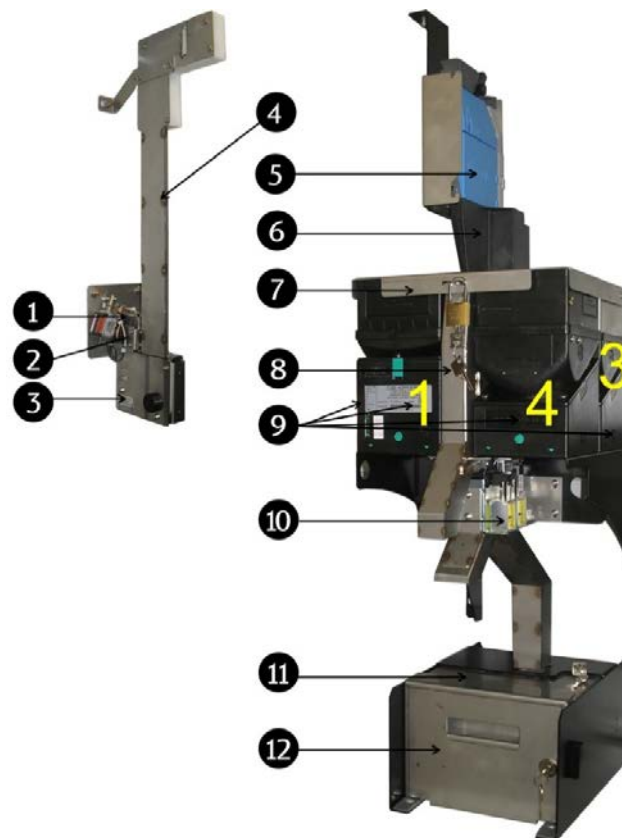
Fig. 77: MVE; on the door (left), inside the device (right)
