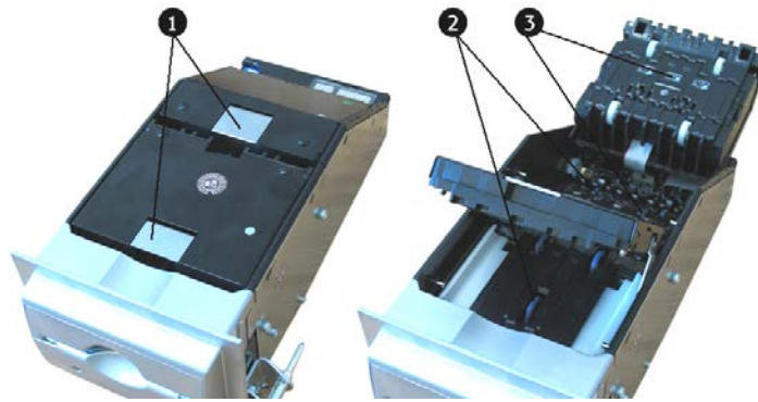
Fig. 91: Cleaning the banknote reader
