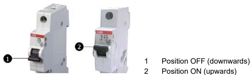
Fig. 18: Automatic circuit breaker, position OFF and ON
