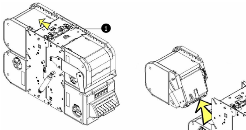
Fig. 96: Removing the recycling or (multi-)escrow cassettes
