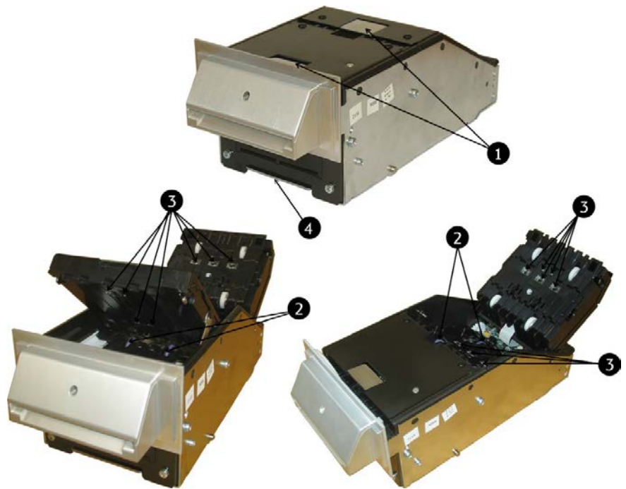
Fig. 87: Cleaning the MFL
