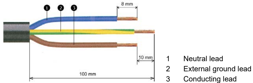
Fig. 34: Removing the insulation
