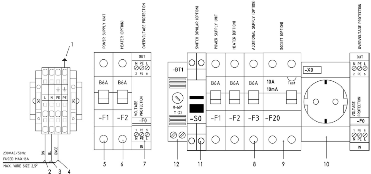
Fig. 33: Terminal block -X0, power distribution box (basic equipment and with optional components)
