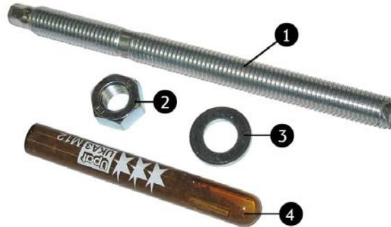
Fig. 26: Designa mounting kit
