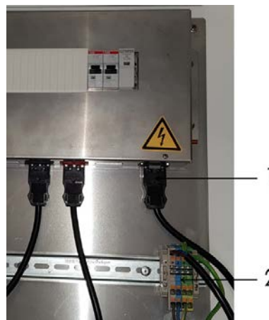
Fig. 20: Terminal block -X0
