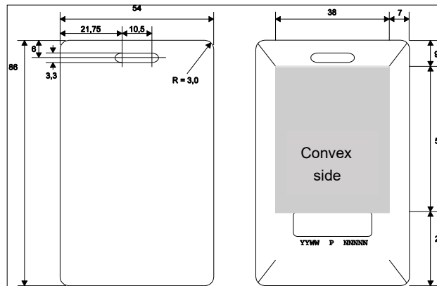
Fig. 113: EasyMove card (active): Approx. dimensions in mm
