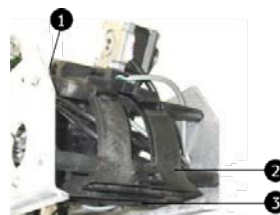
Fig. 43: Feeding unit and rear parking position
