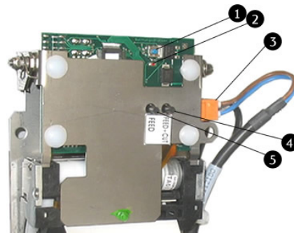
Fig. 74: PCB receipt printer
