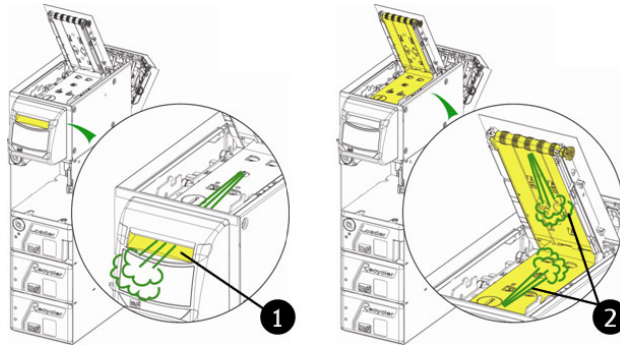
Fig. 99: Cleaning the banknote acceptor and the positioner
