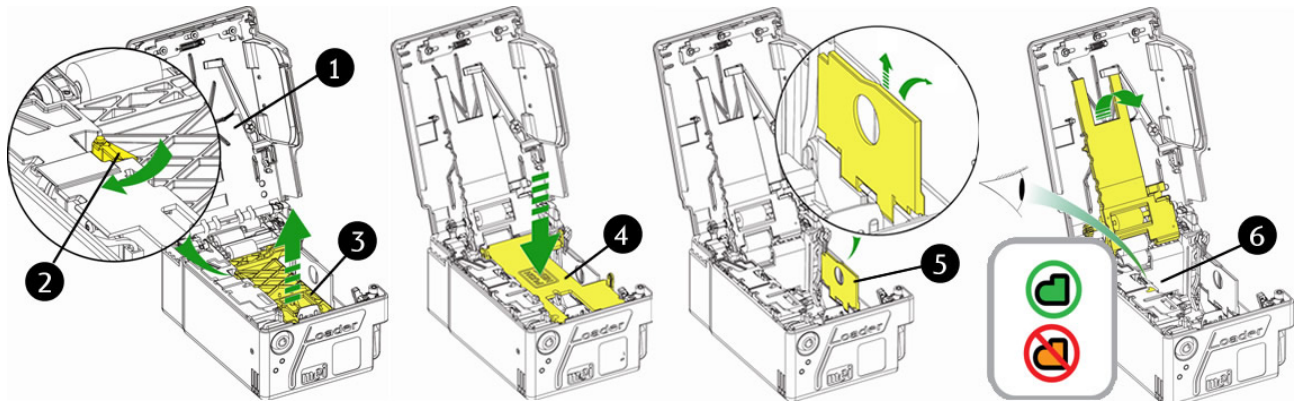
Fig. 96: Filling with banknotes
