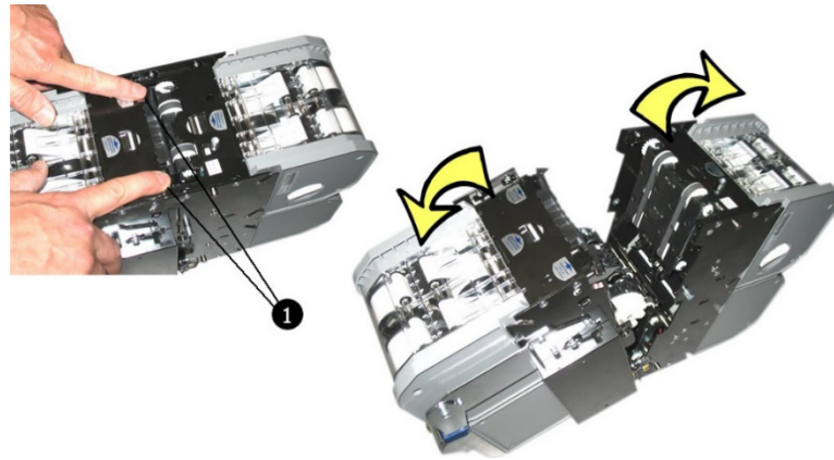
Fig. 82: Opening the chassis
