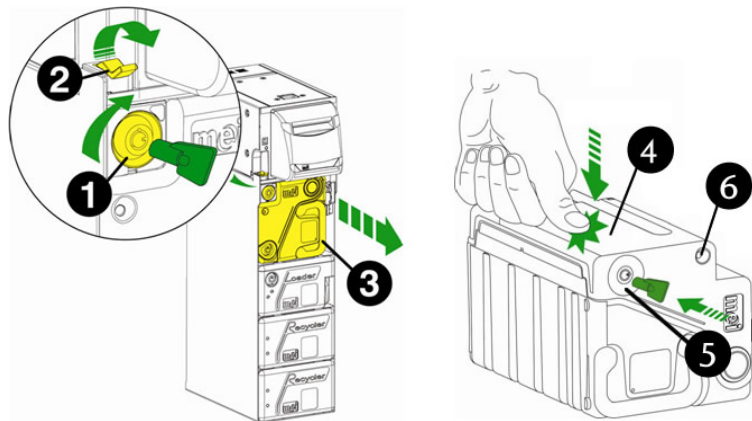
Fig. 92: Removing and opening the banknote cassette
