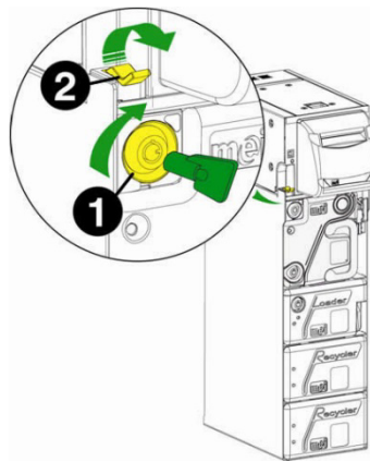
Fig. 91: Locking mechanism
