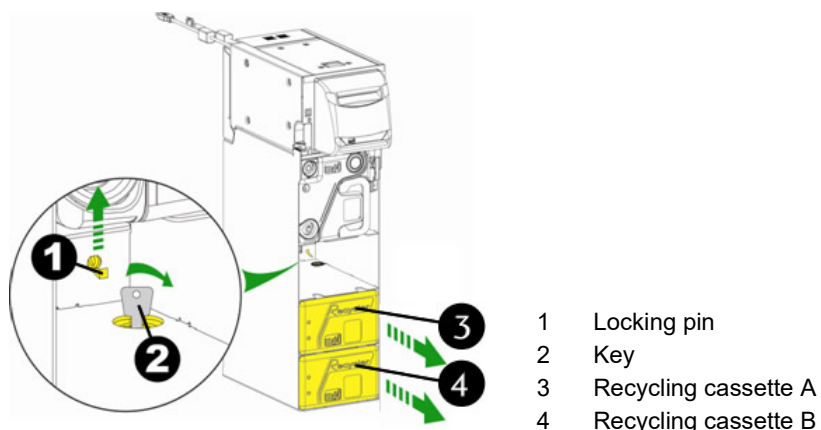
Fig. 105: Removing the recycling cassette
