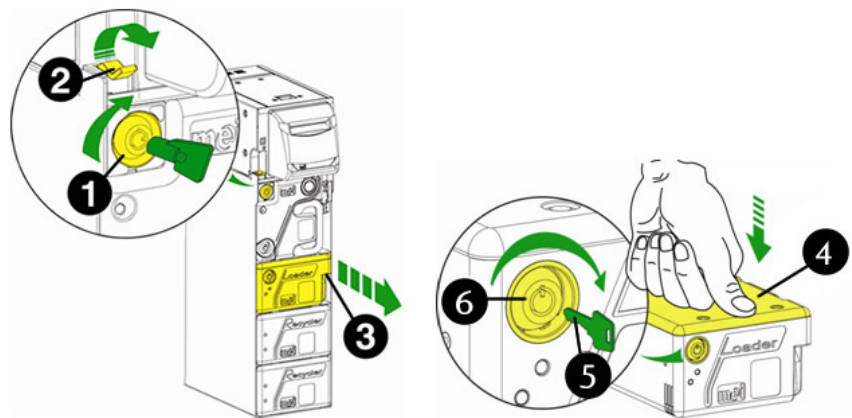
Fig. 93: Removing and opening the loader cassette
