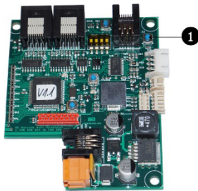
Fig. 69: Test ticket button
