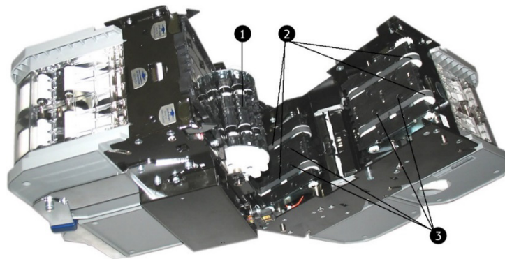
Fig. 83: Cleaning the chassis
