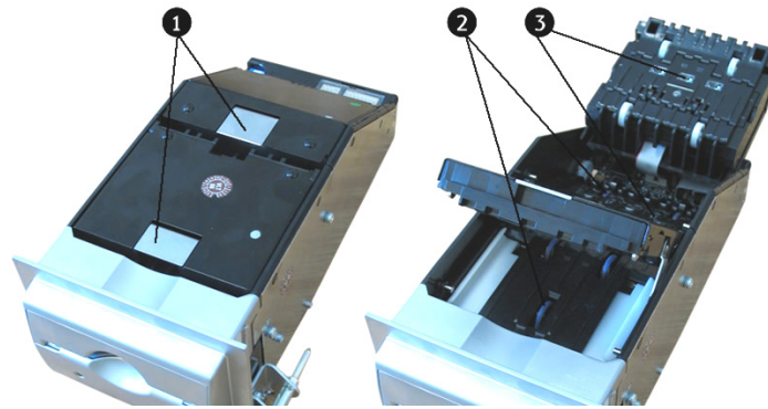
Fig. 80: Cleaning the banknote reader
