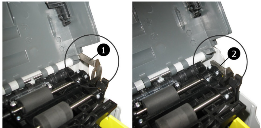
Fig. 94: Loader cassette, locking latch: correct position (left), wrong position (right)
