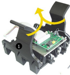
Fig. 56: Clamp attachment
