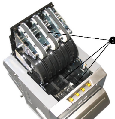
Fig. 89: Cleaning the dispensing cassette
