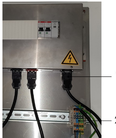
Fig. 22: Terminal block -X0
