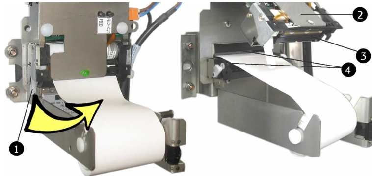
Fig. 76: Releasing the opening lever to loosen the print head from the paper reel
