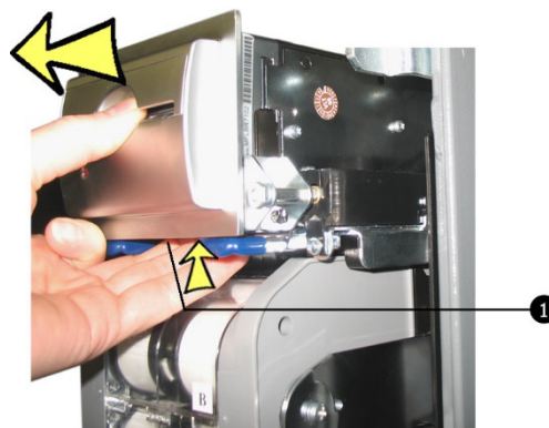
Fig. 79: Removing the banknote reader
