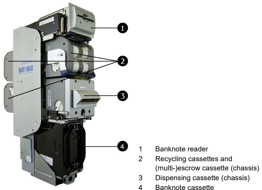
Fig. 77: Banknote recycler BNR CASHCODE
