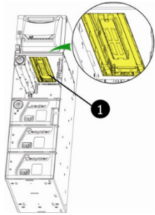
Fig. 104: Banknote cassette-pressure plate
