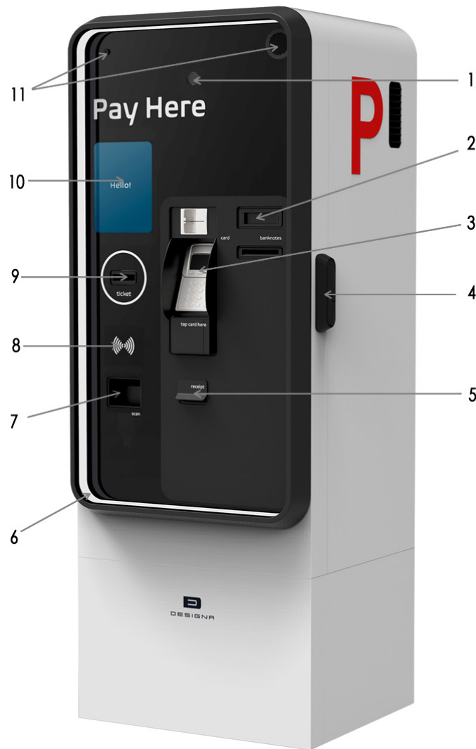
Fig. 8: Components on the door (figure with options)
