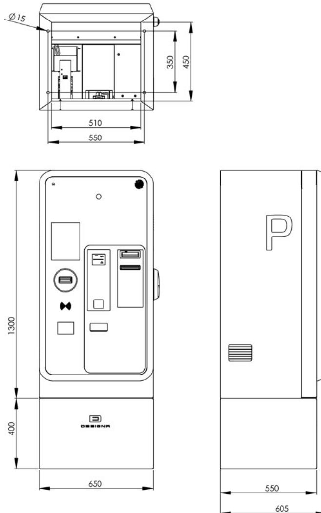
Fig. 6: Pay Coinless, with optional illuminated frame, dimensions in mm
