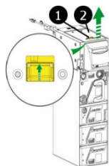
Fig. 98: Opening the positioner cover
