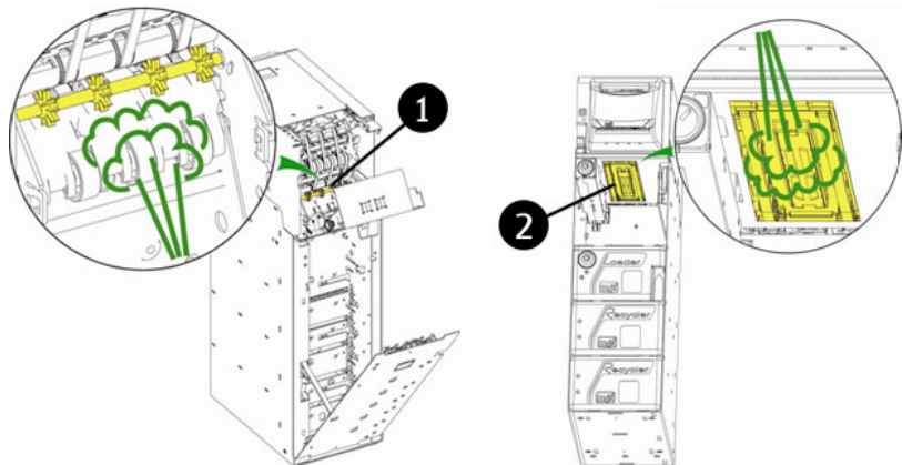
Fig. 102: Cleaning the test unit and the main module from the bottom
