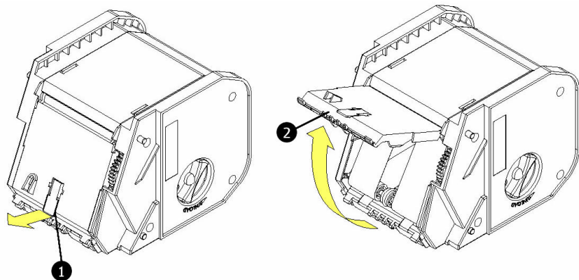
Fig. 86: Opening the recycling or (multi-)escrow cassettes
