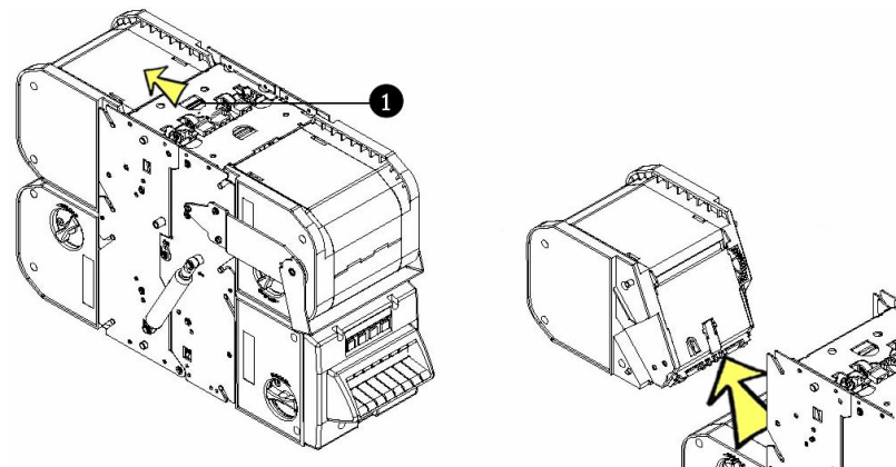
Fig. 85: Removing the recycling or (multi-)escrow cassettes
