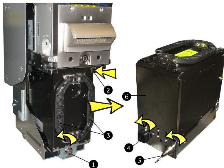
Fig. 78: Removing and opening the banknote cassette
