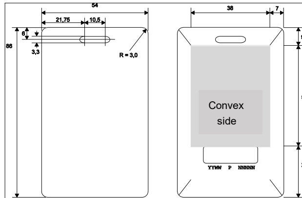
Fig. 108: EasyMove card (active): Approx. dimensions in mm
