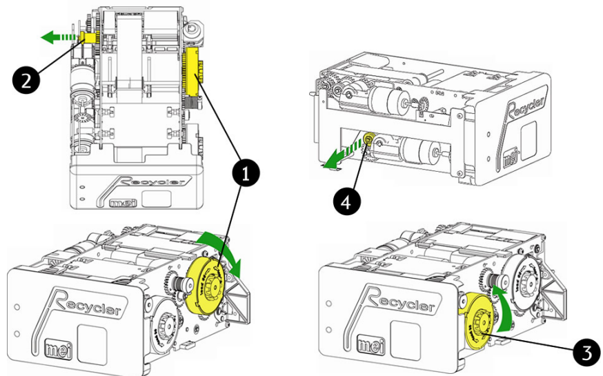
Fig. 106: Recycling cassette: Removing trapped banknotes
