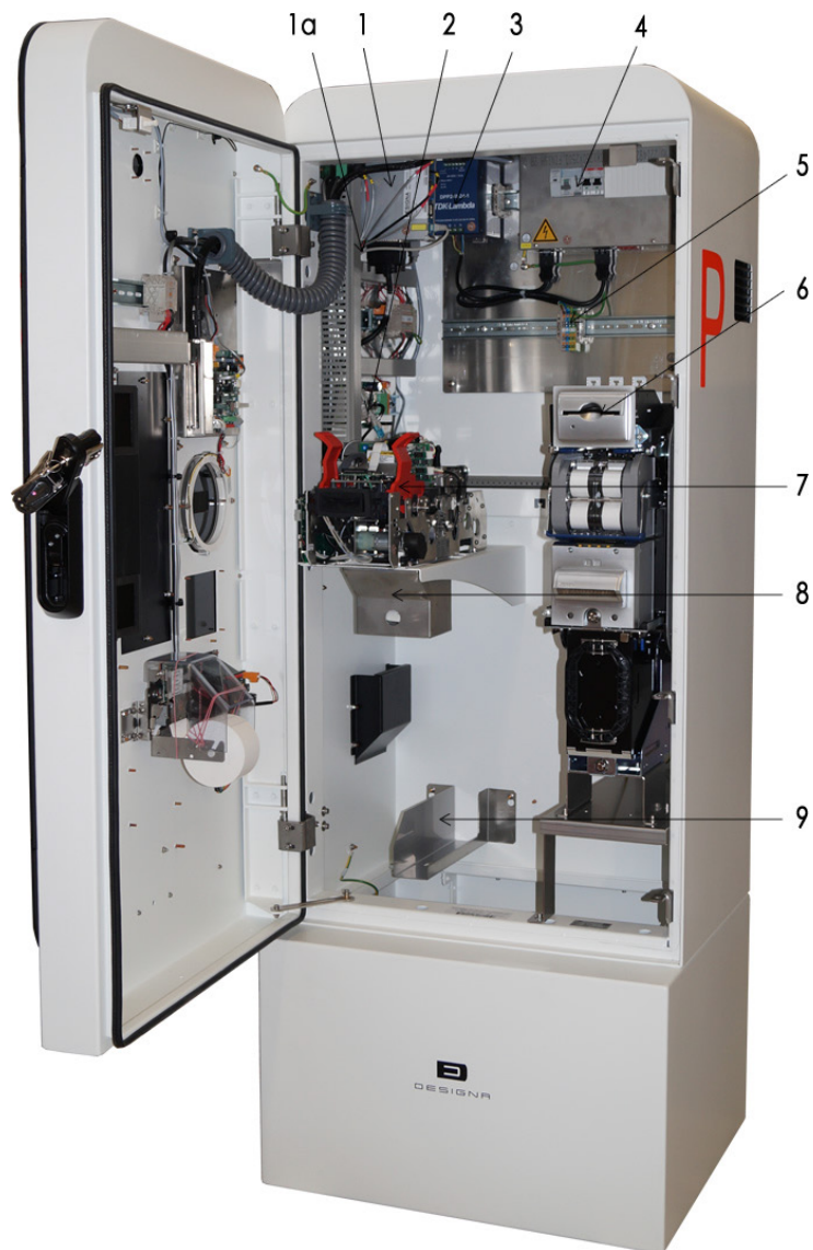
Fig. 11: Components inside the device (figure with options)
